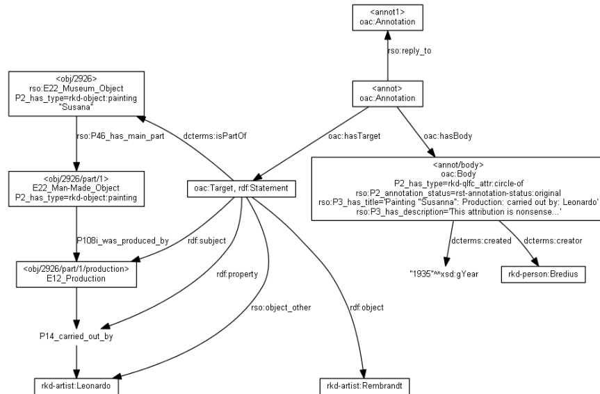
Fig. 5. Using RDF Reification and OAC in ResearchSpace
