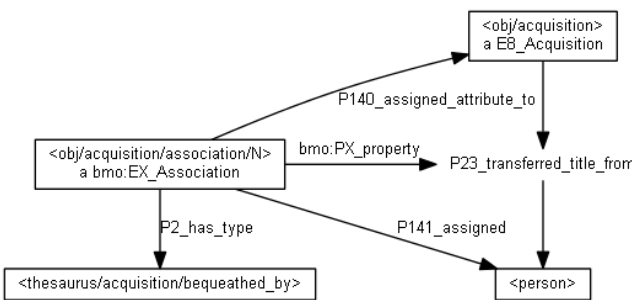
Fig. 6. Representing Bequeathal Using EX_Association and PX_property
